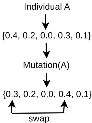
Fig. 4: Mutation Example
