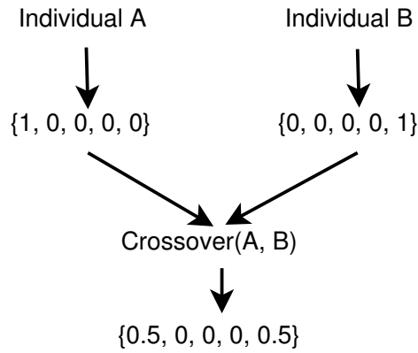
Fig. 3: Crossover Example
