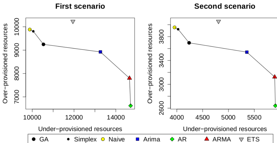
Fig. 19: Solutions for the Fifa World Cup series.
