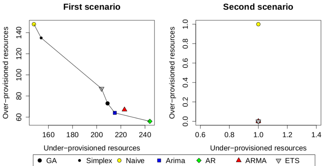
Fig. 18: Solutions for NASA series.
