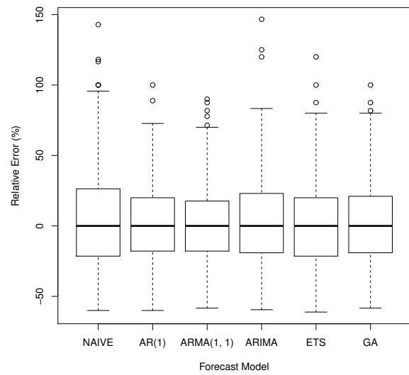
Fig. 9: Forecast Error ClarkNet Log With Outliers.
