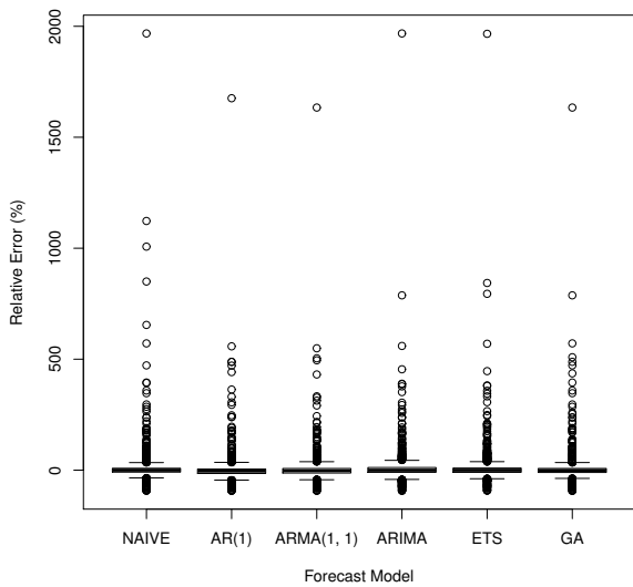
Fig. 15: Forecast Error Fifa World Cup 98 Log With Outliers.
