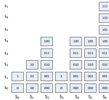
Figure 7: Encoding Space of Antibodies
