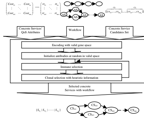
Figure 1: Overview of the HIAWSC Framework
