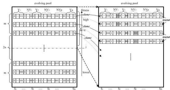
Figure 9: The process of the Heuristic Immune Algorithm for Web Service Composition: The left side shows antibodies before evolution, the right side antibodies mutated with vaccines.
