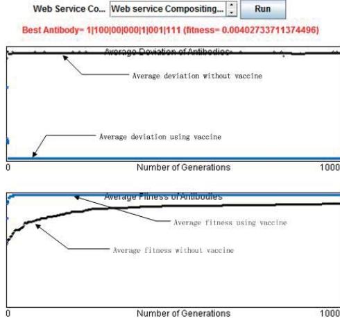
Figure 8: Results of Experiments with N_S = 10
